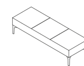
SYM3BEN Symbol 3 Seat Bench mm W1530 D510 H410 Seat 410 inch W60 D20 H16 Seat 16
