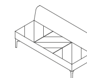
HAT3NA Hatch 3 Seater no arms mm W 1530 D 690 H 685 Seat 410 inch W 60 D 27 H 27 Seat 16
