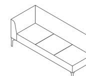
SYM3RA Symbol 3 Seater right arm mm W1710 D690 H685 Seat 410 inch W67.5 D27 H27 Seat 16
