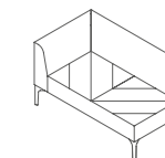
HAT2RA Hatch 2 Seater right arm mm W 1200 D 690 H 685 Seat 410 inch W 47 D 27 H 27 Seat 16
