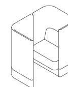
PULPHRAP Pullman Chair Pod with Upholstered Plinth Screen right mm W 900 D 1300 H 1300 Seat 450 inch W 35.5 D 51 H 51 Seat 18
