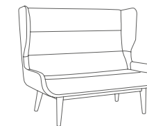
HSH2SFBWD Hush 2 Seat Sofa with Wooden Base mm W 1350 D 815 H 1160 Seat 430 inch W 53 D 32 H 45.5 Seat 17
