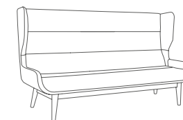
HSH3SFBWD Hush 3 Seat Sofa with Wooden Base mm W 2000 D 815 H 1160 Seat 430 inch W 79 D 32 H 45.5 Seat 17
