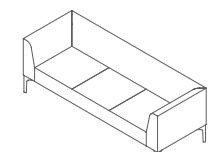
SYM32A Symbol 3 Seater 2 arms mm W1890 D690 H685 Seat 410 inch W74.5 D27 H27 Seat 16
