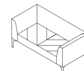
HAT22A Hatch 2 Seater 2 arms mm W 1380 D 690 H 685 Seat 410 inch W 54.5 D 27 H 27 Seat 16
