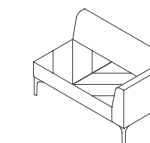
HAT2LA Hatch 2 Seater left arm mm W 1200 D 690 H 685 Seat 410 inch W 47 D 27 H 27 Seat 16
