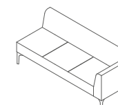
SYM3LA Symbol 3 Seater left arm mm W1710 D690 H685 Seat 410 inch W67.5 D27 H27 Seat 16
