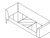
HAT32A Hatch 3 Seater 2 arms mm W 1890 D 690 H 685 Seat 410 inch W 74.5 D 27 H 27 Seat 16
