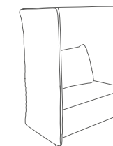
CLOP15H Cloud Plain 1.5 Seat Sofa with High Back mm W 1100 D 750 H 1300 Seat 400 inch W 43.5 D 29.5 H 51 Seat 15.5
