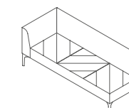
HAT3RA Hatch 3 Seater right arm mm W 1710 D 690 H 685 Seat 410 inch W 67.5 D 27 H 27 Seat 16
